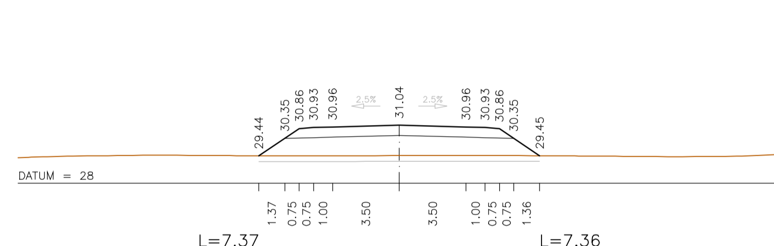
km=3+875
