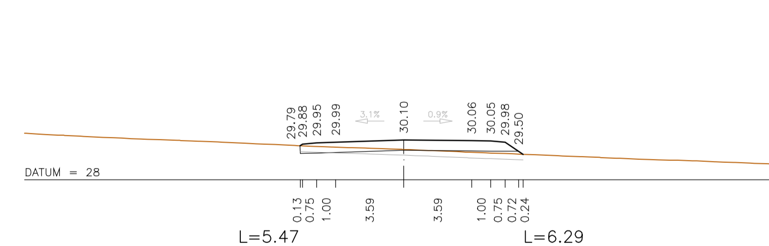
km=4+000
