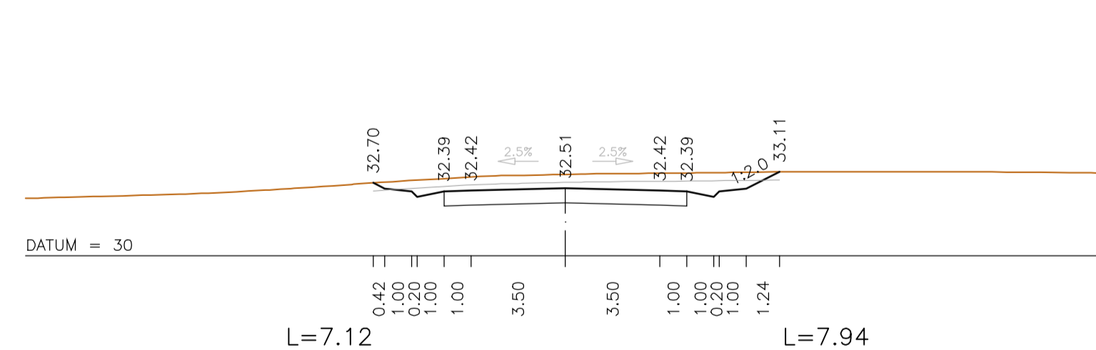
km=3+825
