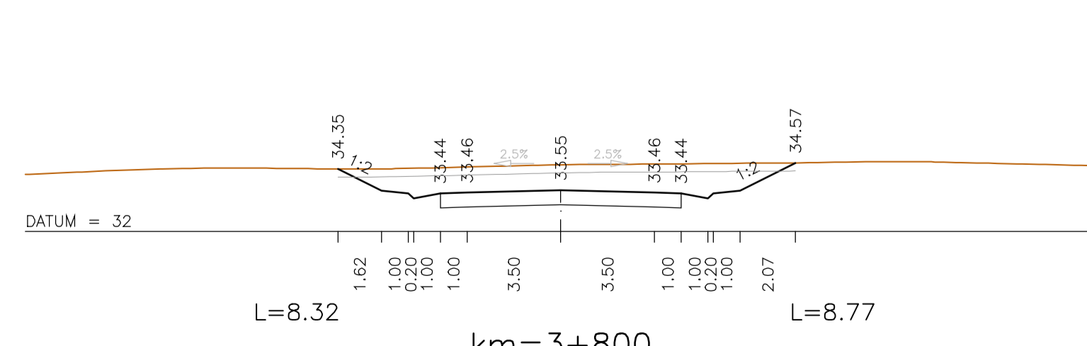
km=3+800
