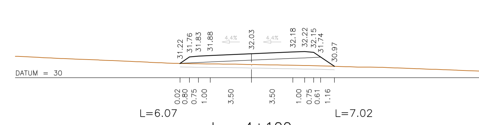
km=4+100
