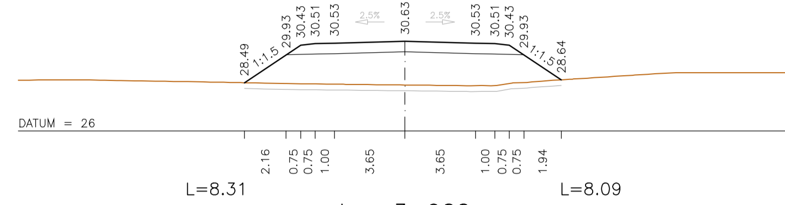
km=3+900
