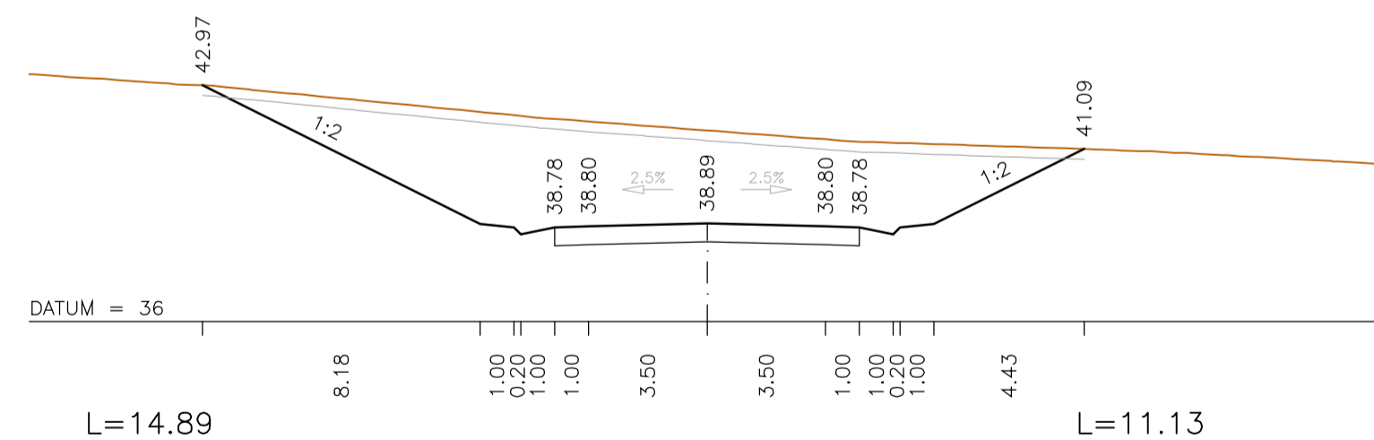
km=3+675
