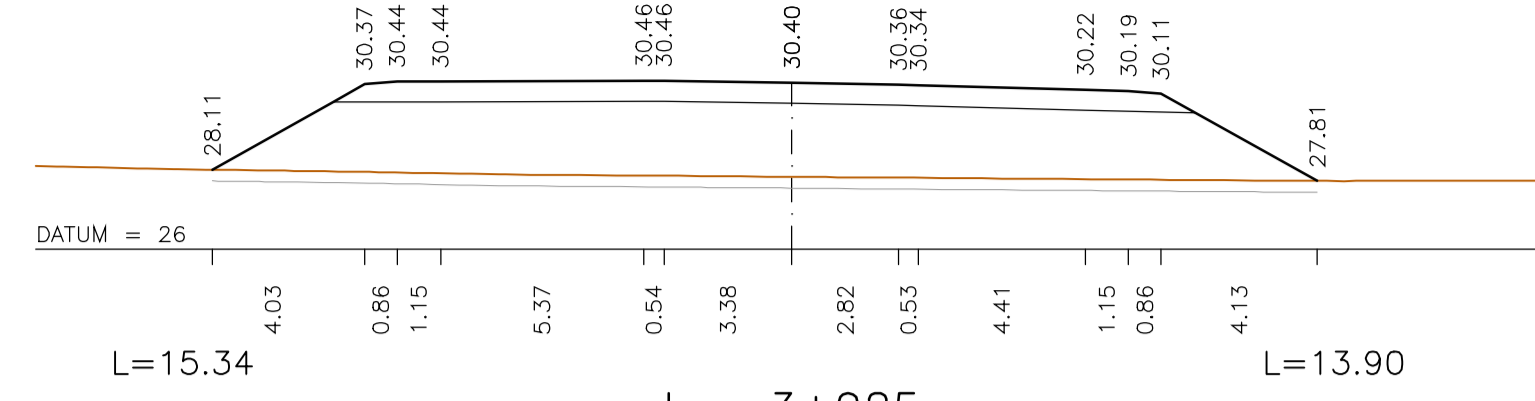
km=3+925
