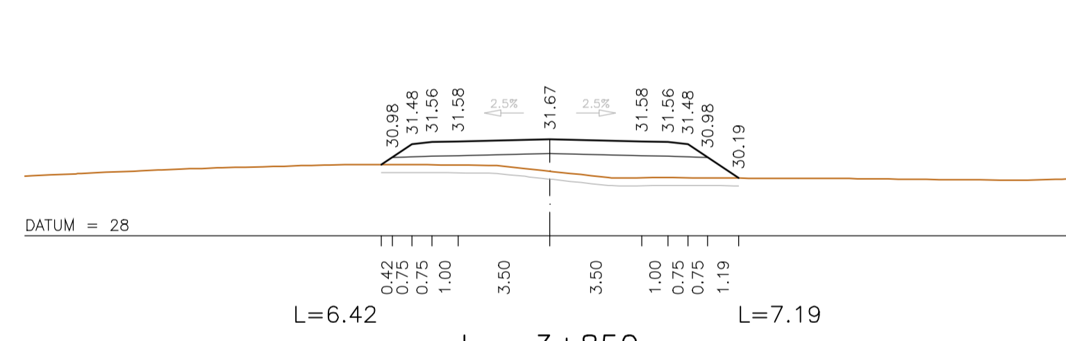
km=3+850
