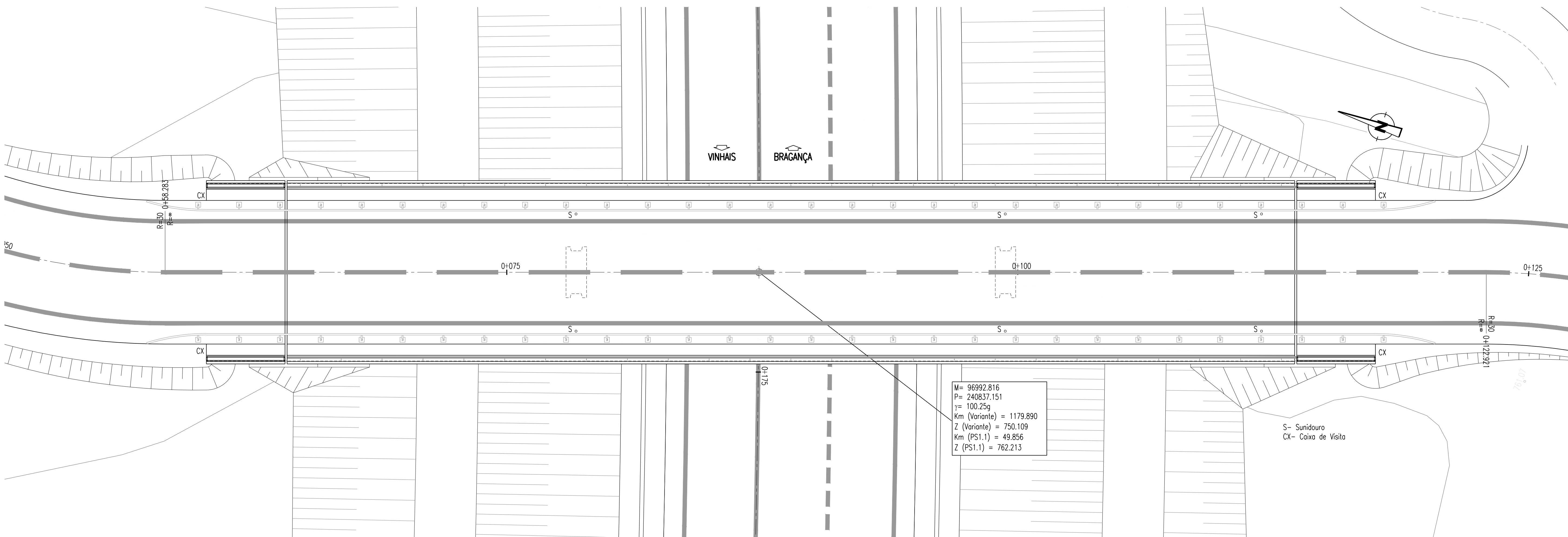
PLANTA A1=1:100/A3=1:200
