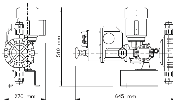
SINGLE PUMP - Electric Actuator Adjustment
