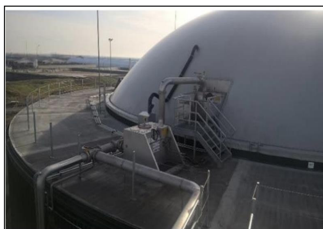
Figura III.7 – Digestor Triton
