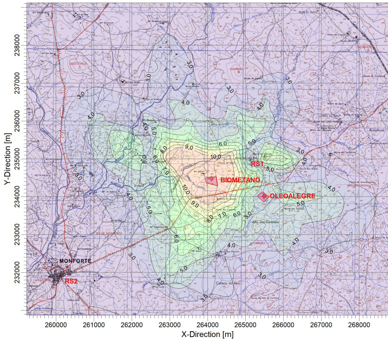
PLOT FILE OF HIGH 1ST HIGH 1-HR VALUES FOR SOURCE GROUP: ALL Max: 14,5 [ug/m 3 ] at (263500,00, 235000,00) ug/m 3
