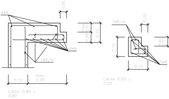
PORMENOR DA TAMPA COM GRELHA/Detail of the Lid with Grate
